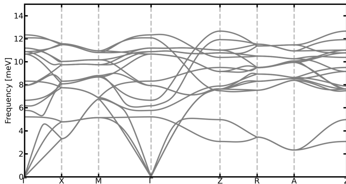
Fig. 1. Phonon spectra of U_3Si_2 . The lines represent the ABINIT calculation, whilst the dots are experimental results.
