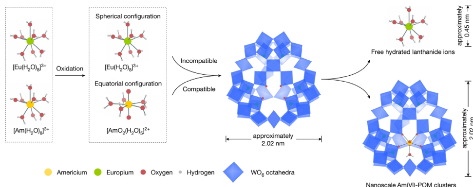
Fig. 1. Schematic illustration of the frame of the ultrafiltration separation of nanoscale Am(VI)-POM clusters from lanthanides
