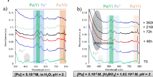
Figure 1: UV-Vis-NIR spectra of Pu(IV) solution a) in water and b) in boric acid.
