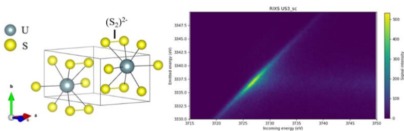
Fig. 1. Crystal structure and U 3d4f RIXS map of US_3 ( P2_1/m )
