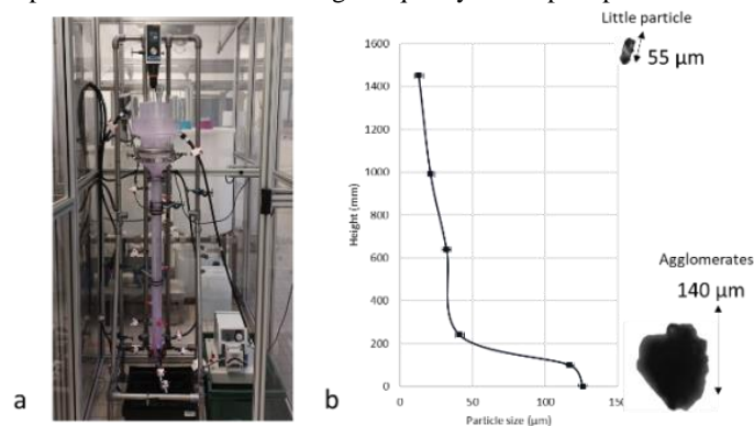
Fig. 1 : Photograph of the fluidized bed (a) and particle size distribution along the column (b)
