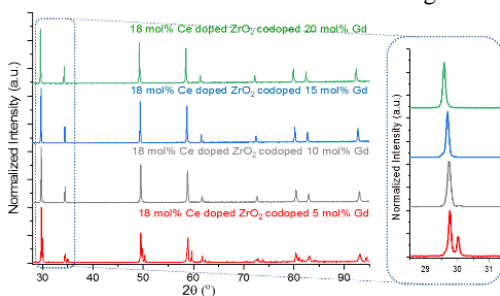
Fig. 1. XRD diffractograms of zirconia doped with 18 mol% Ce, co-doped with 5, 10, 15 or 20 mol% Gd
